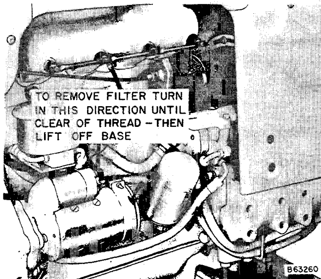
Figure 5 - Oil Filter (Diesel Engine)
