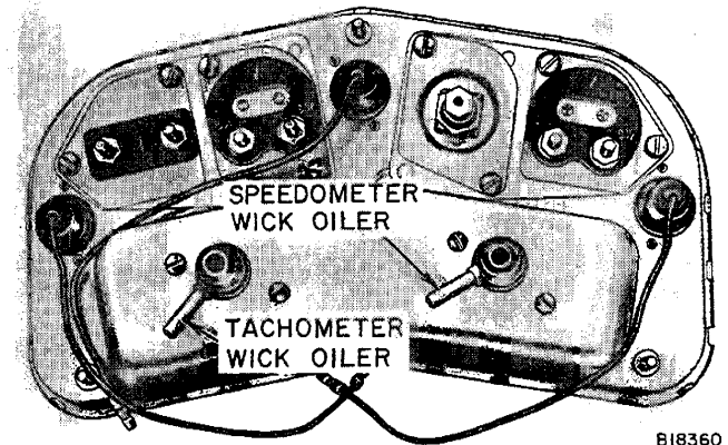
Figure 10 - Instrument Wick Oilers
