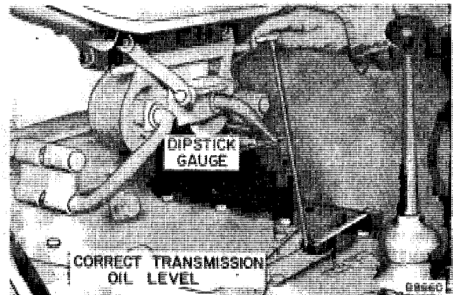
Figure 11 - Checking Transmission and Final Drive Oil Level
